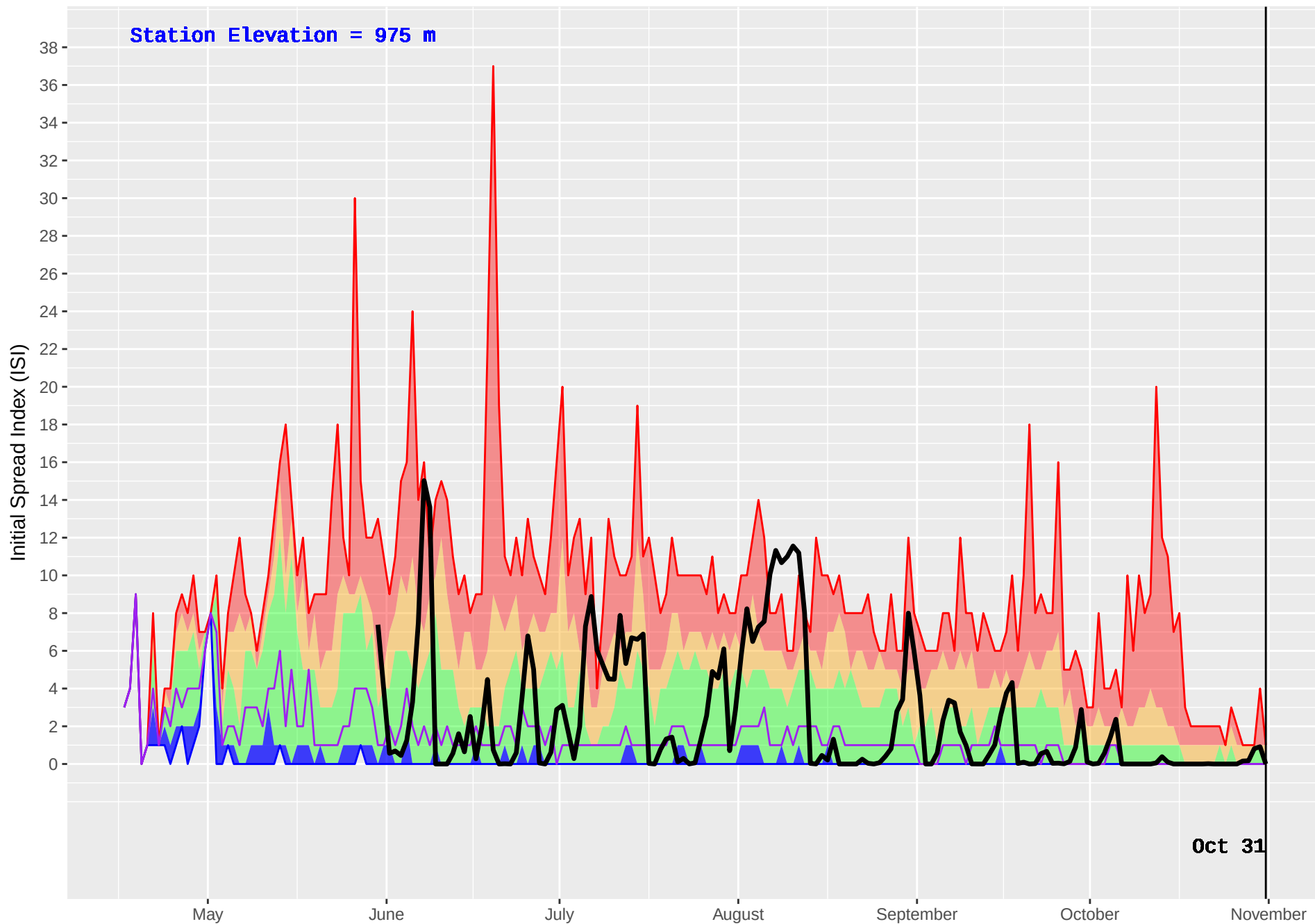
MCGREGOR 2 (192) : Historical (1986–2016) and Current (2017) Noon Initial Spread Index (ISI)
