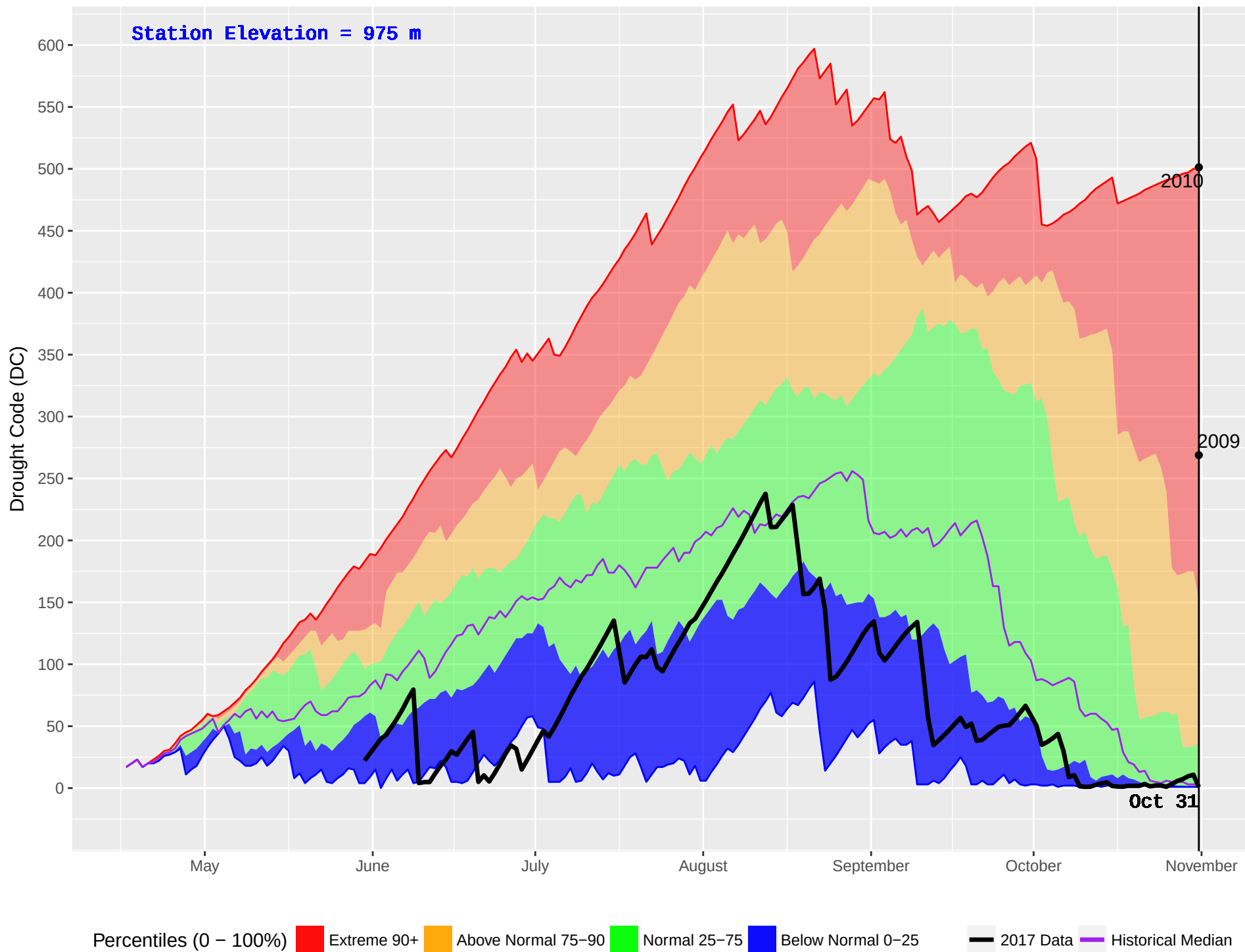
MCGREGOR 2 (192) : Historical (1986–2016) and Current (2017) Noon Drought Code (DC)
