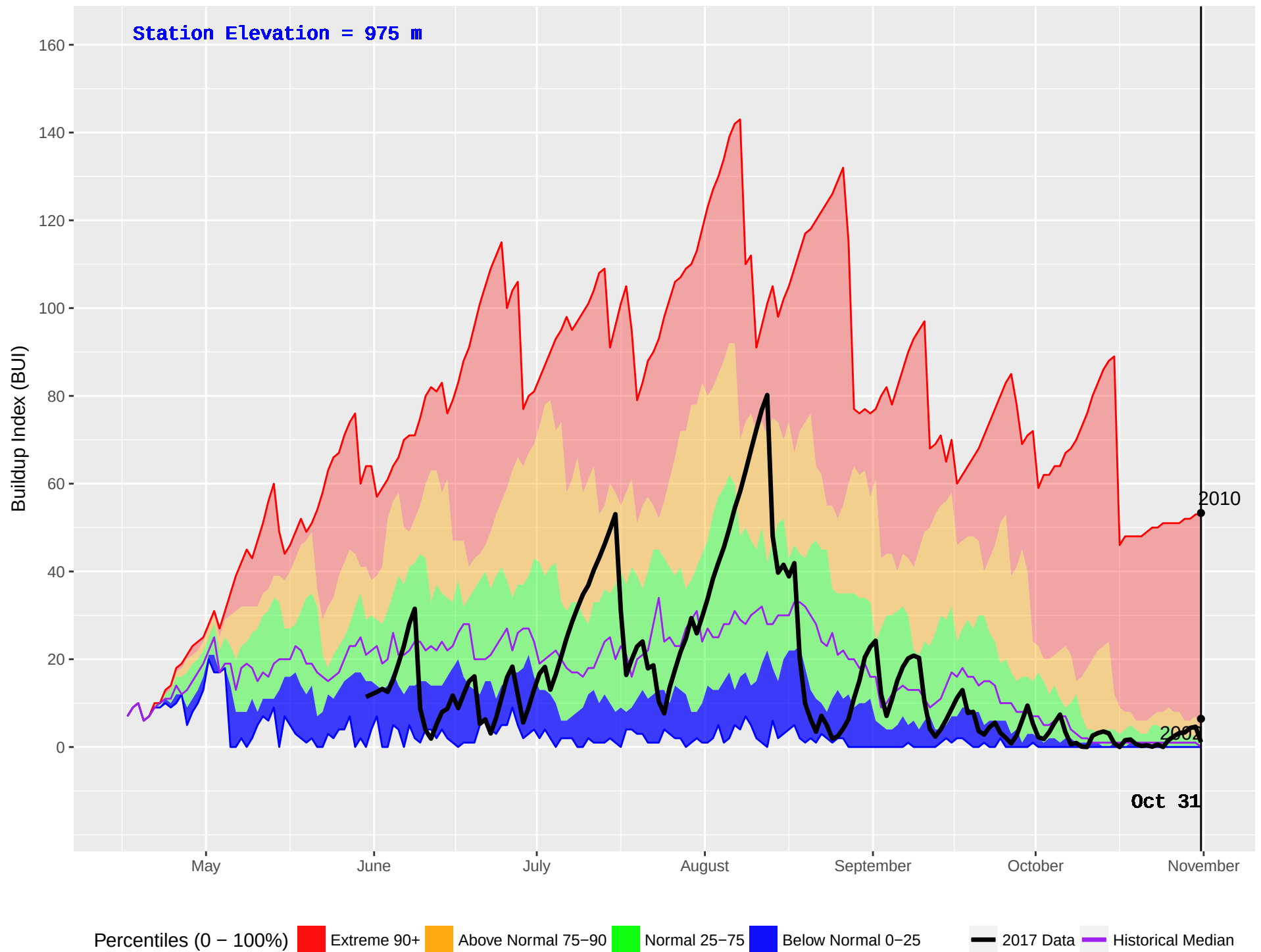
MCGREGOR 2 (192) : Historical (1986–2016) and Current (2017) Noon Buildup Index (BUI)
